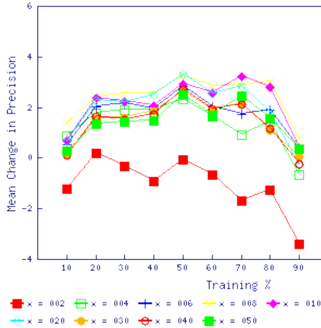
Figure 3. Mean difference in precision for different values of x
