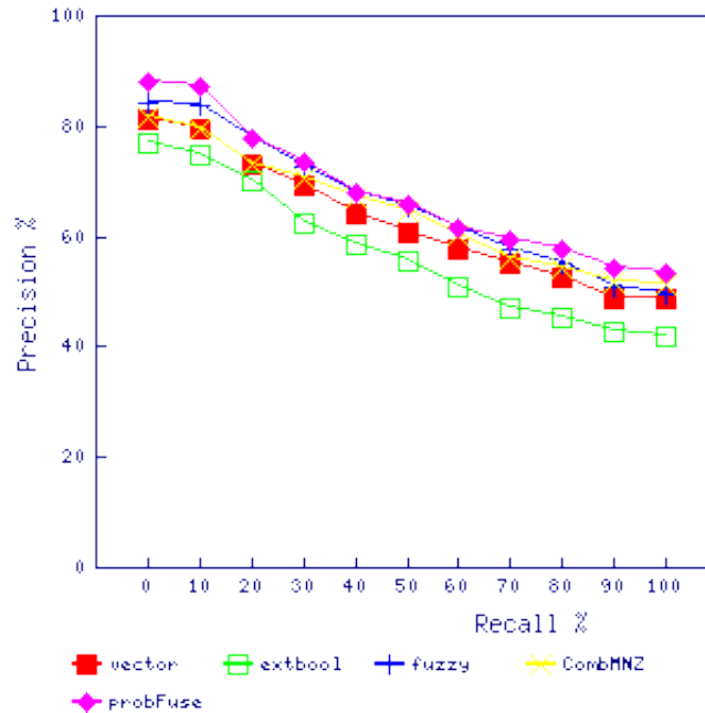
Figure 4. Interpolated Precision graph for the Cranfield collection
