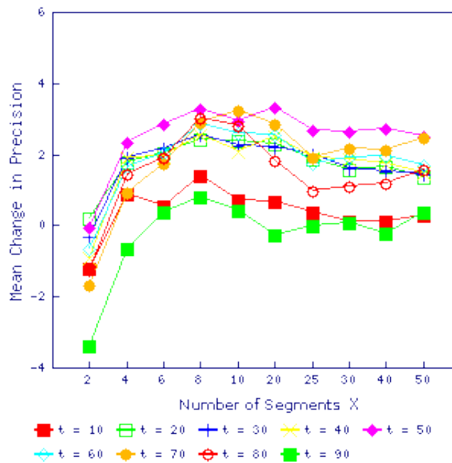
Figure 2. Mean difference in precision for different training set sizes
