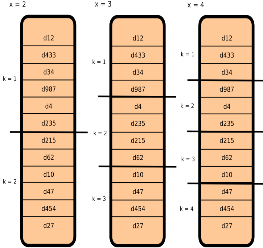
Figure 1. Segmenting a result set for different values of x
